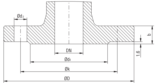
CLASS 150,300,600
