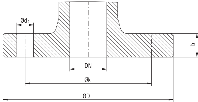
CLASS 125
